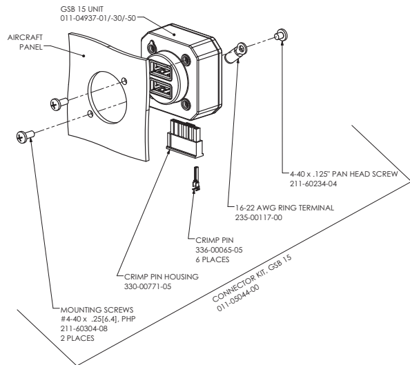
SIDE CONNECTOR (-01/-30/-50 CONFIG) WITH CONNECTOR KIT (011-05044-00) -01 Config Shown
