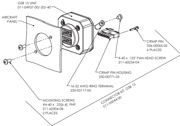
REAR CONNECTOR (-00/-20/-40 CONFIG) WITH CONNECTOR KIT (011-05044-00) -00 Config Shown
