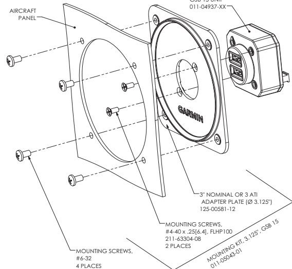
Figure 2-1. GSB 15 Mounting Examples
